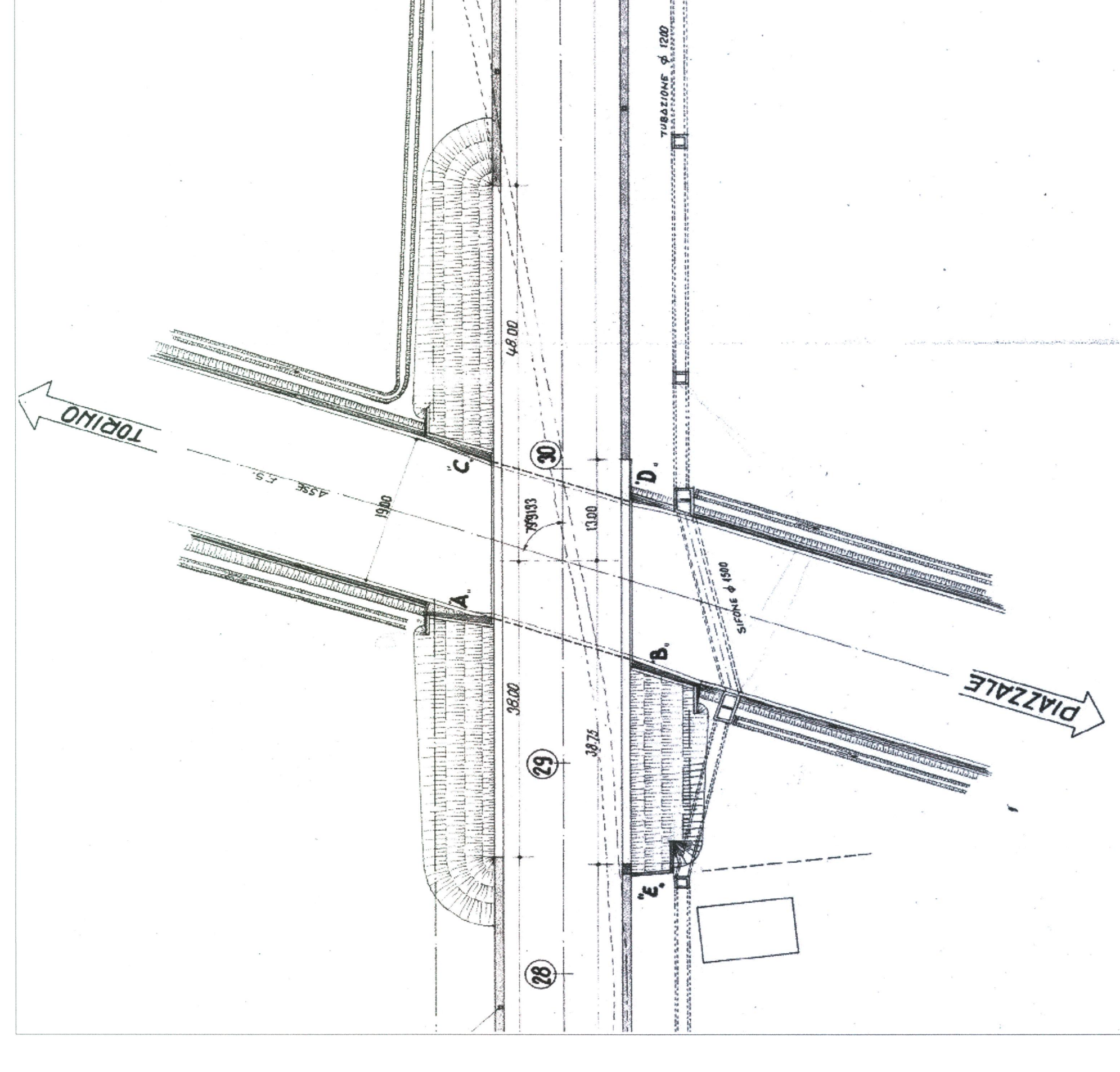
– planimetria –
